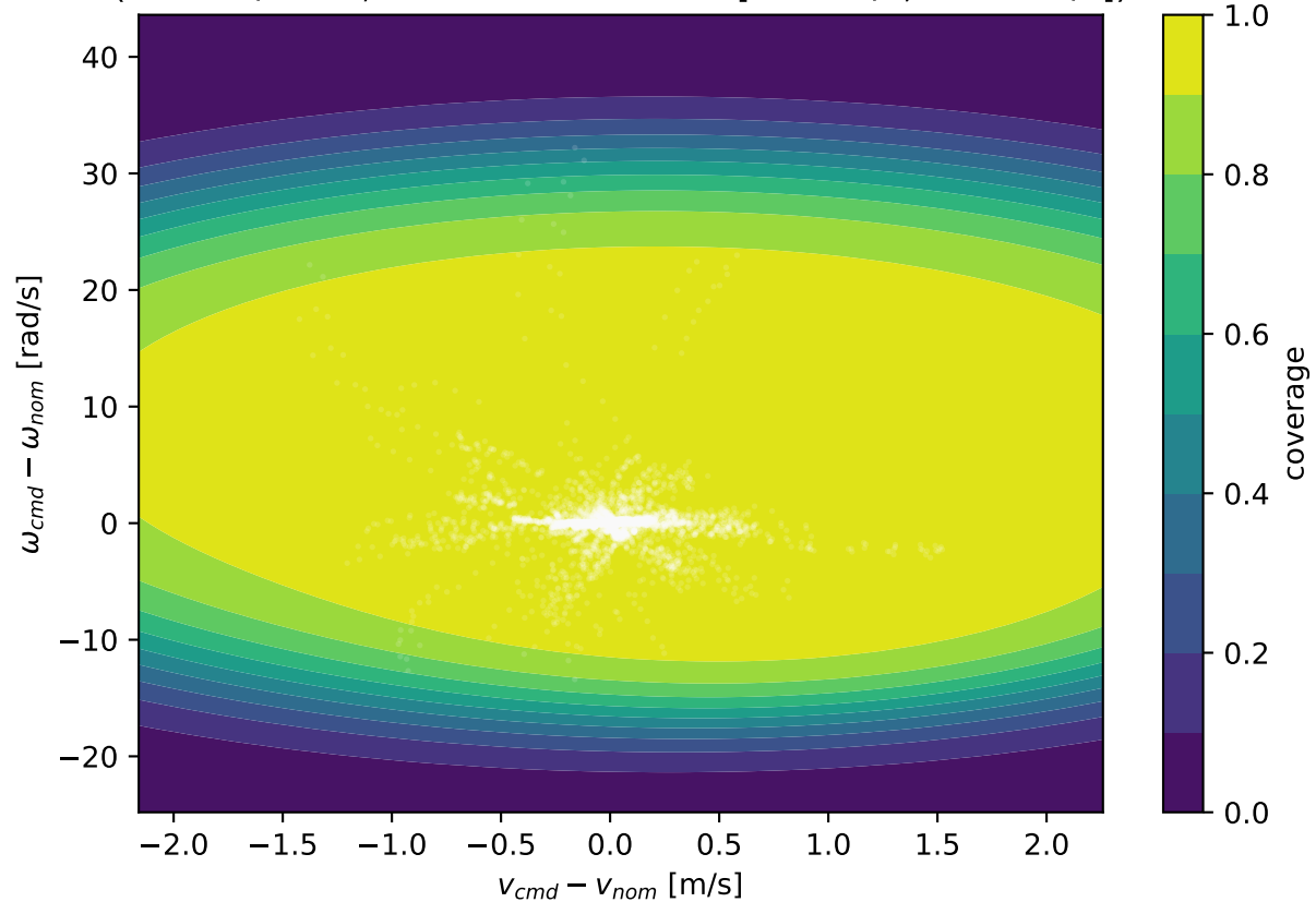
Residual coverage vs command offset (0 = off / OOD; state fixed at mean [0.43 m/s, 0.01 rad/s])
